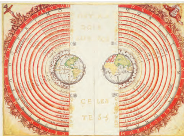
FIGURE 1.12 Illustration of the Geocentric System
