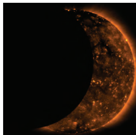
FIGURE 1.6 Solar Eclipse
